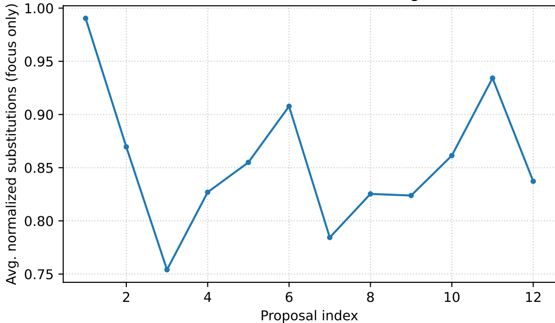
Substitutions over proposals (focus experiments) Qwen3-Next-80B (reasoning)
