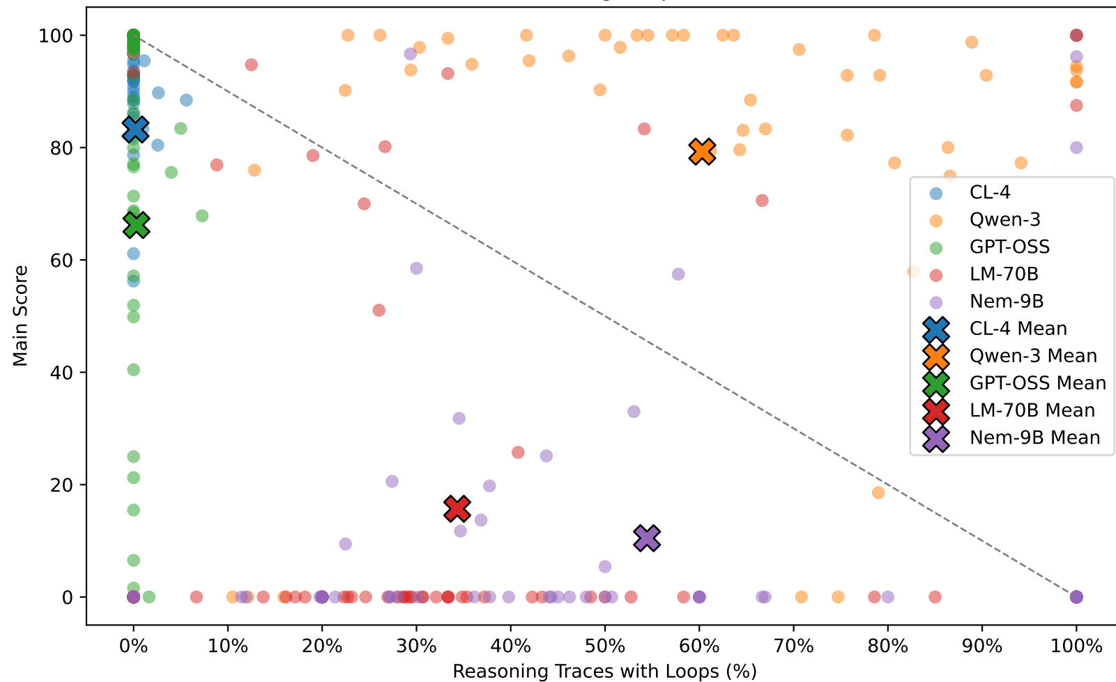
Presence of Reasoning Loops vs Main Score
