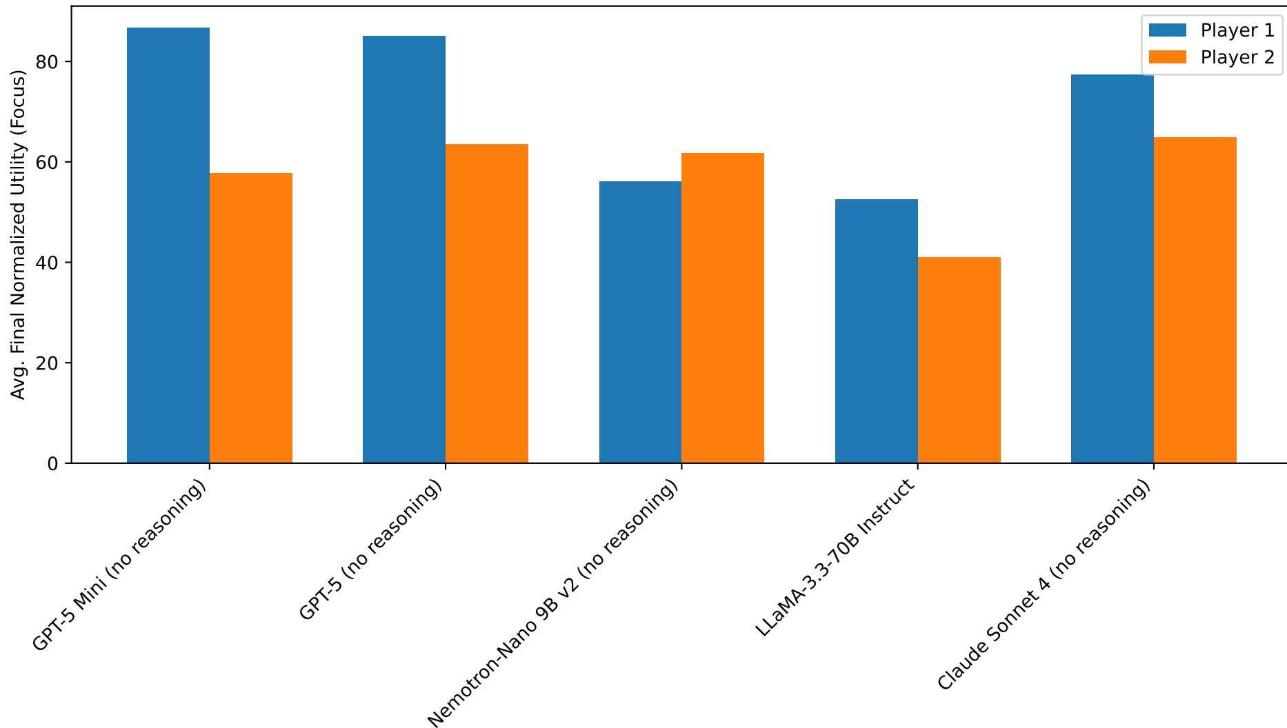
Average Final Scores (Non-Reasoning Models, Focus Experiments)
