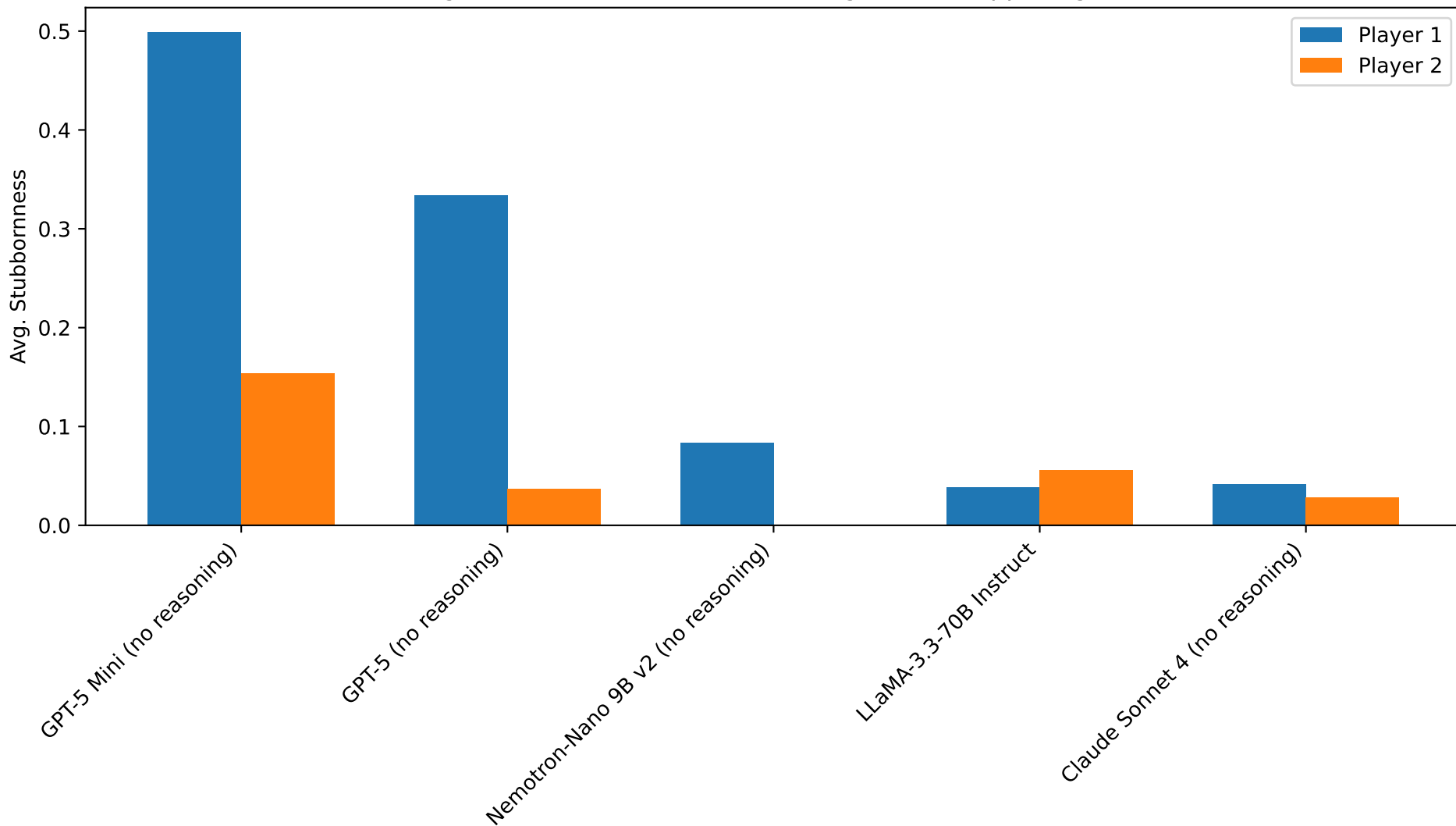
Average Stubbornness (Non-Reasoning Models, Opposing Goals)
