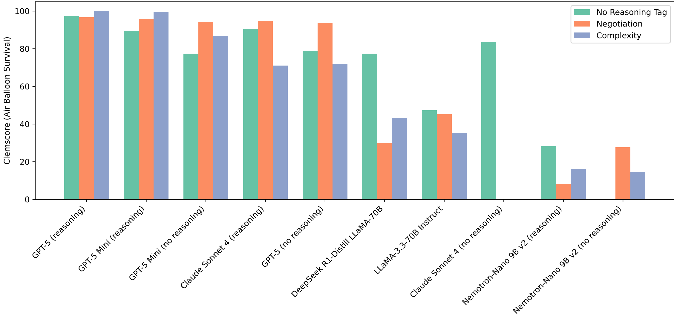
Clemscore by Model and Experiment Type
