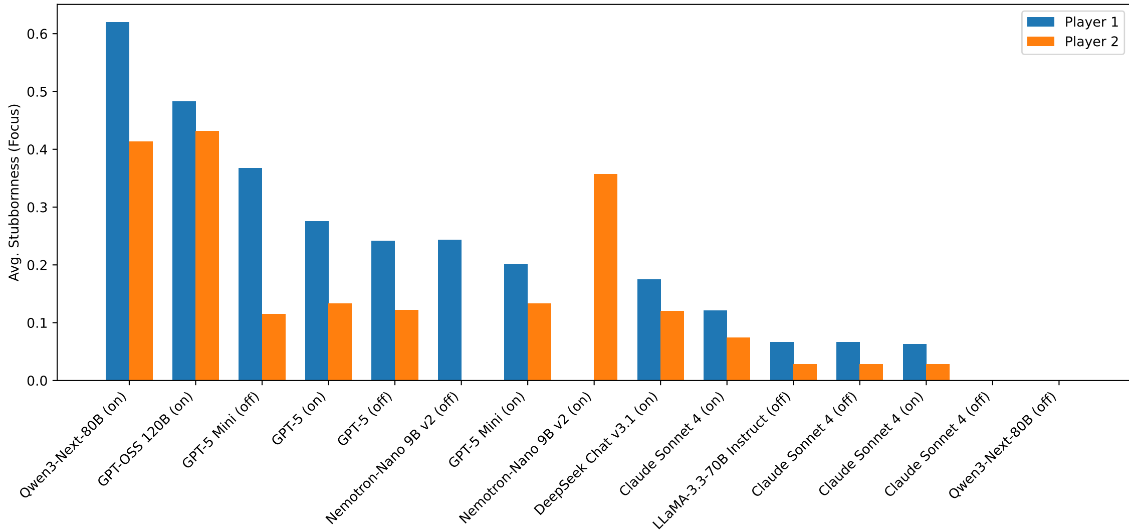
Average Stubbornness by Player (All Models, Focus Experiments)
