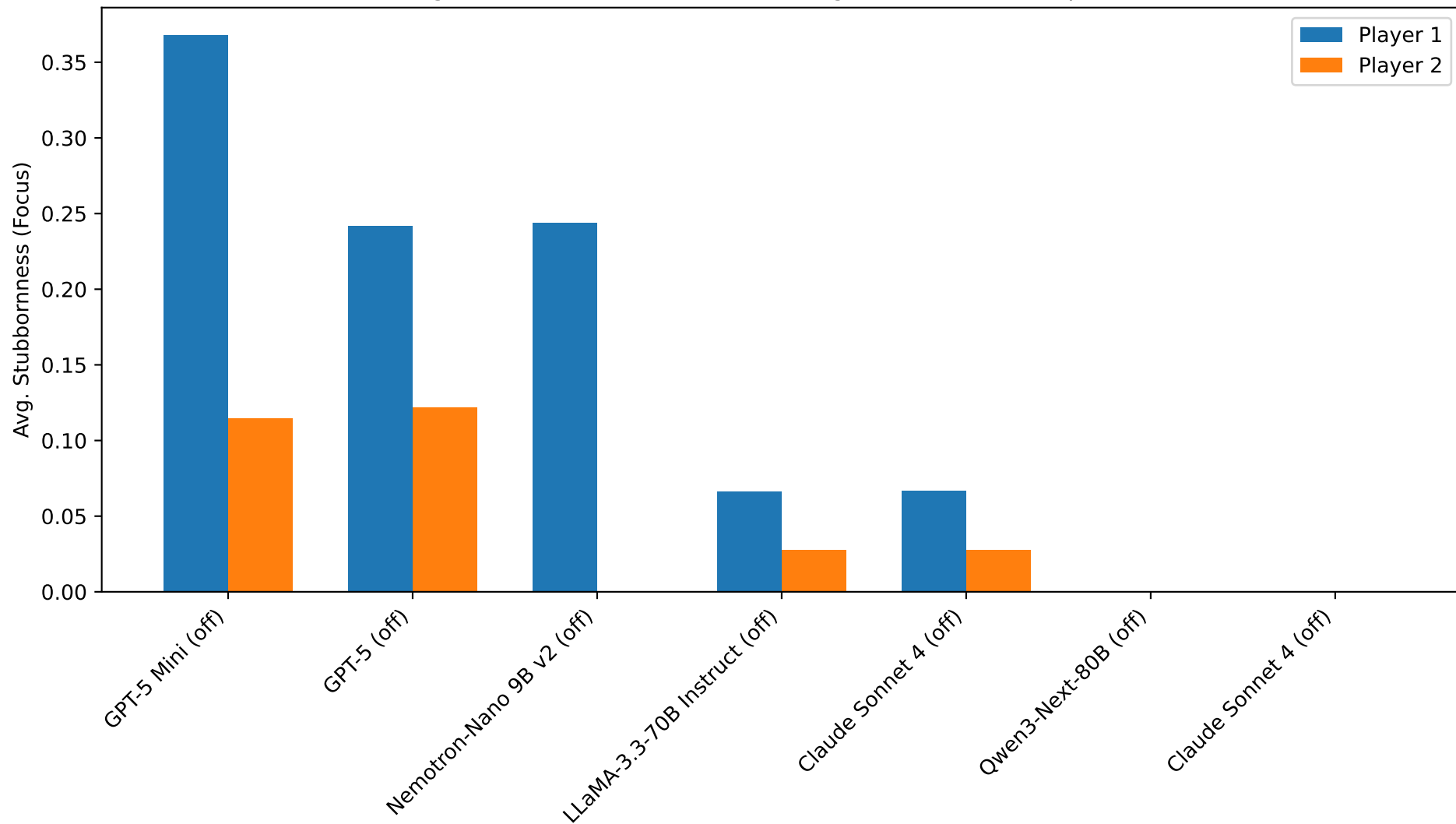
Average Stubbornness (Non-Reasoning Models, Focus Experiments)
