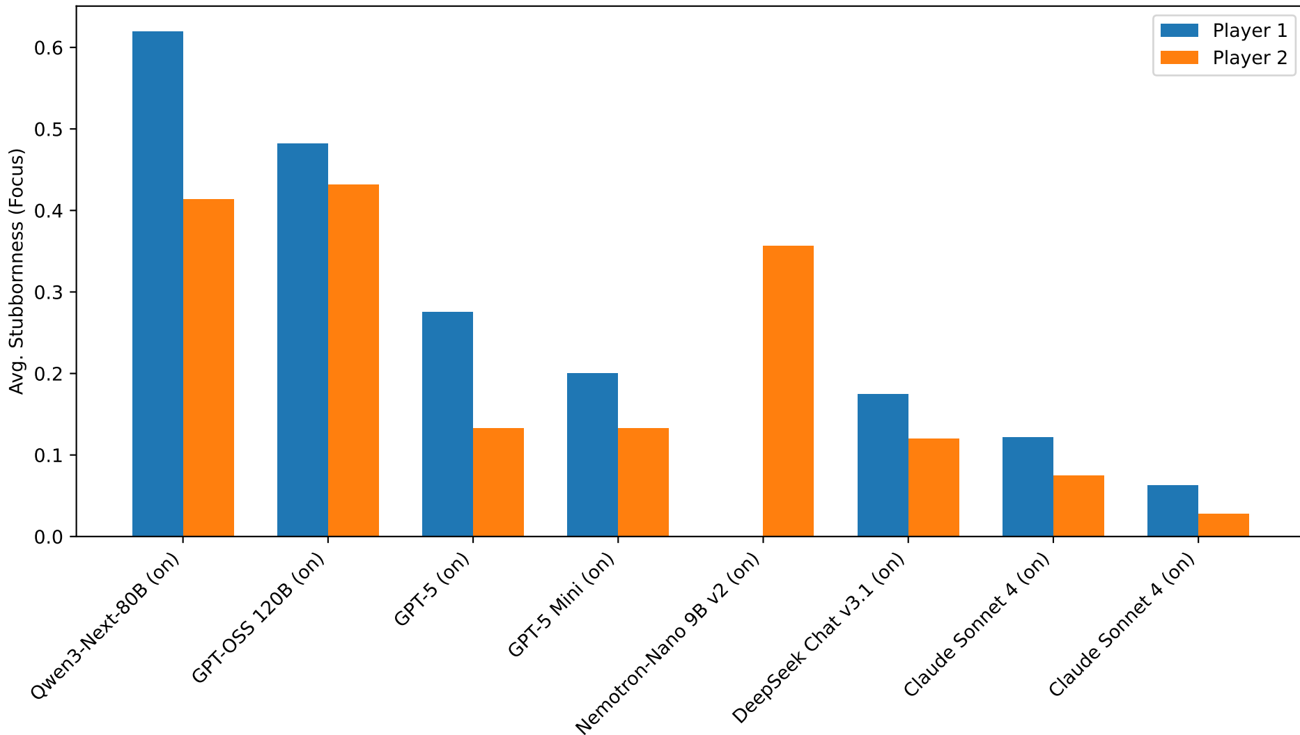
Average Stubbornness (Reasoning Models, Focus Experiments)
