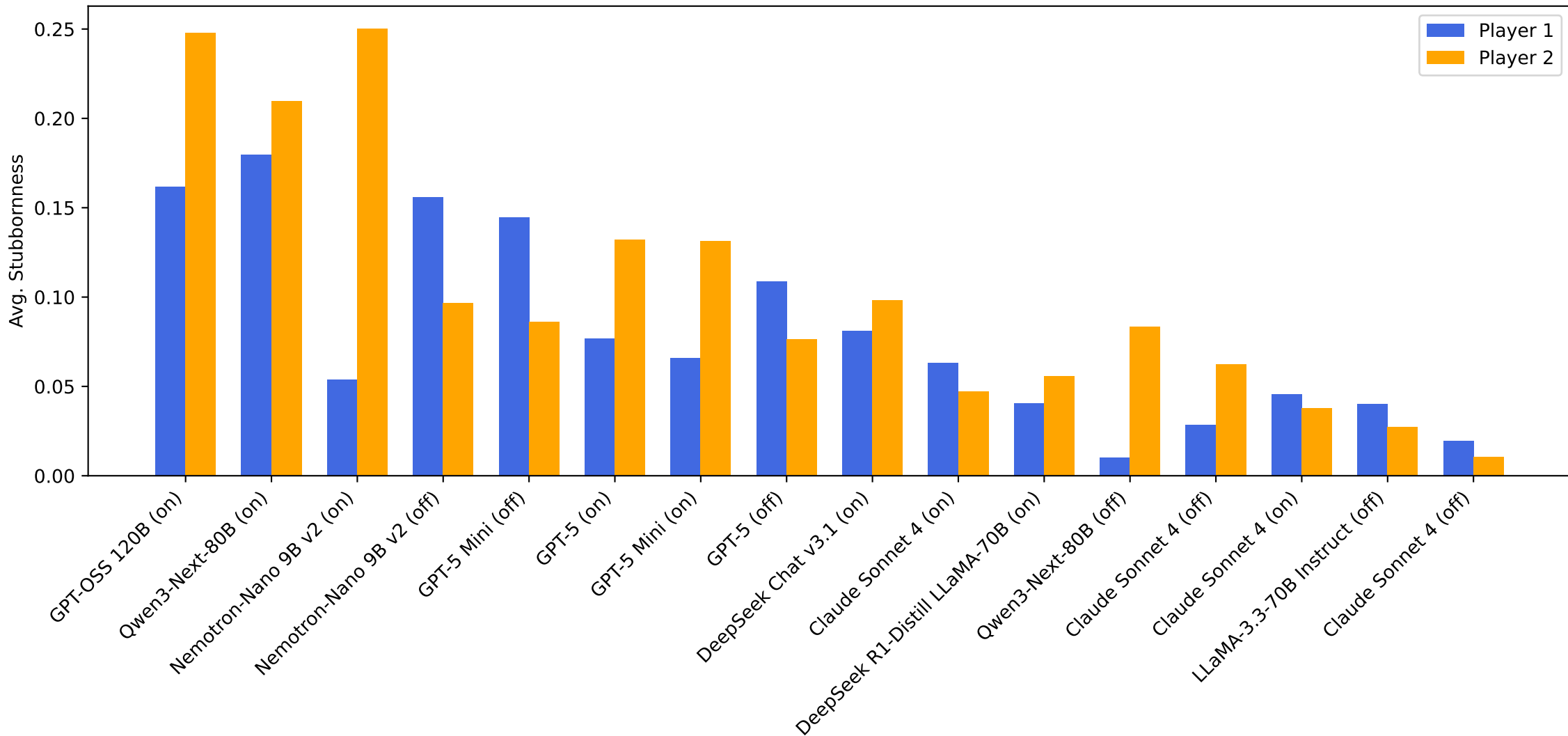
Average Stubbornness per Player Across Models (All Experiments)
