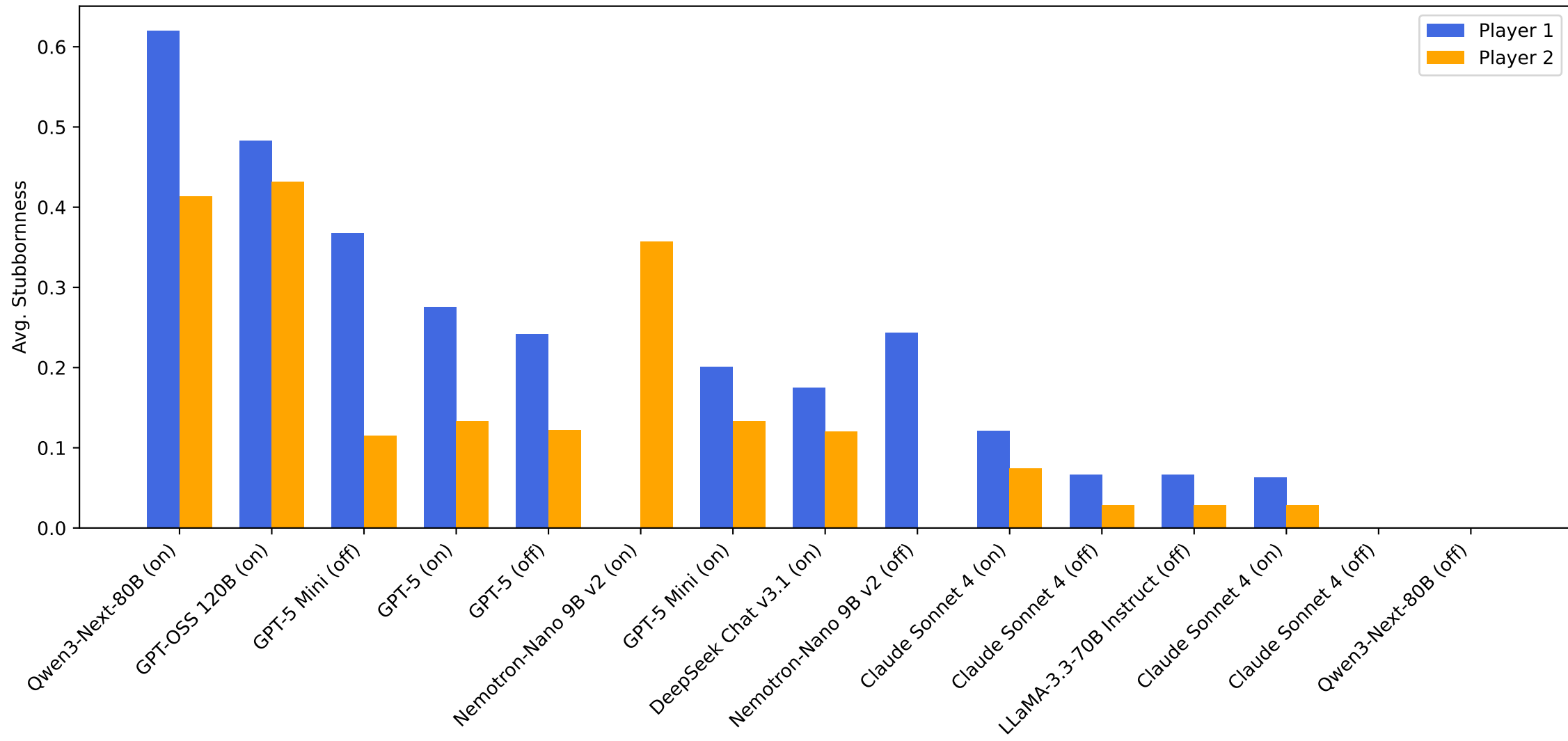
Average Stubbornness per Player Across Models (Focus Experiments)
