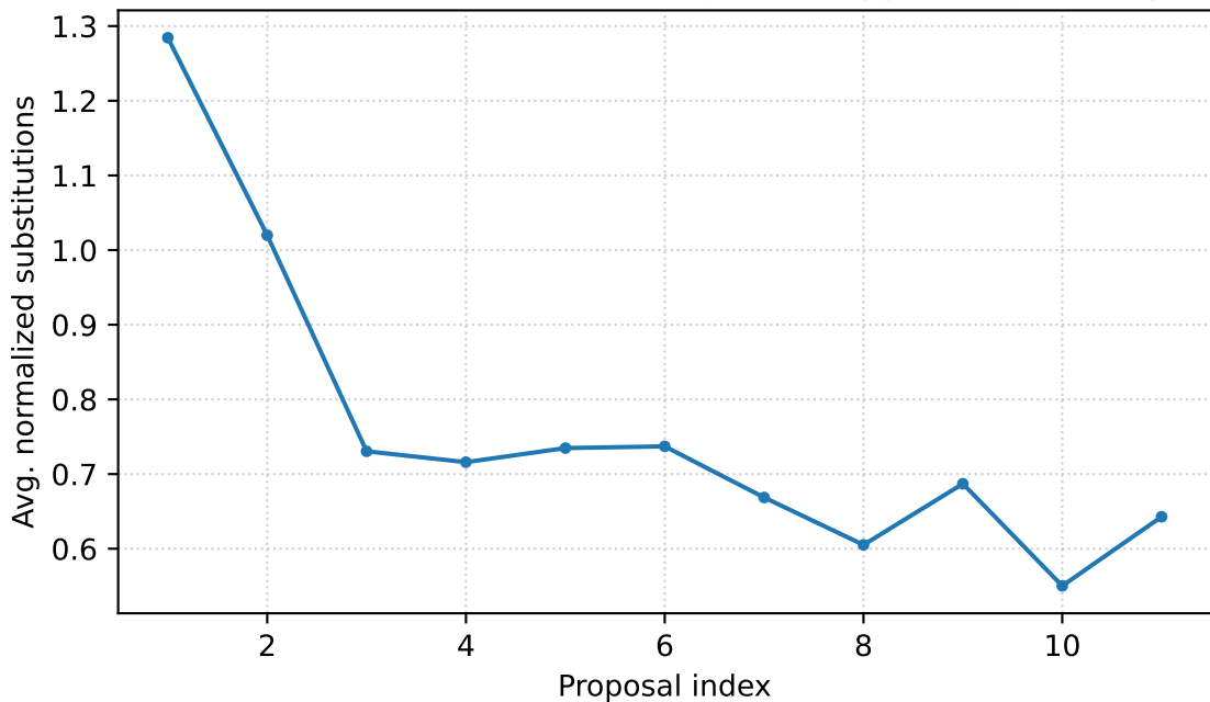
Avg. Normalized substitutions over proposal idx claude-sonnet-4-20250514-no-reasoning-t0.0 - opposite goals experim
