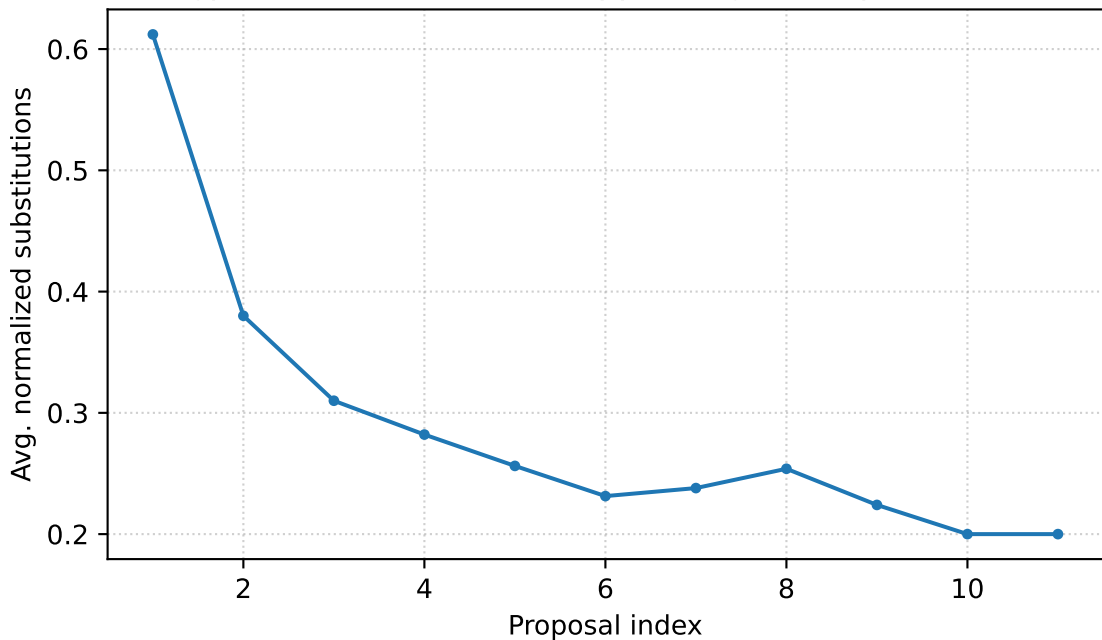
Avg. Normalized substitutions over proposal idx gpt-5-2025-08-07-t1.0 - opposite goals experiments
