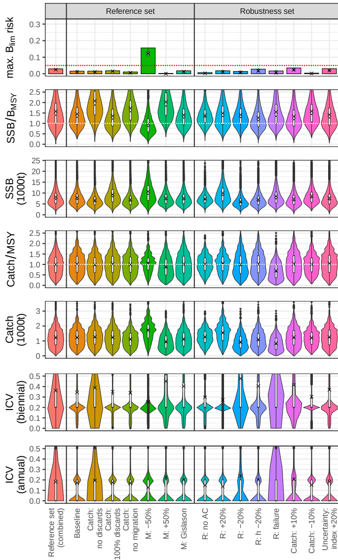
(a) Empirical: chr rule (CHR2)
