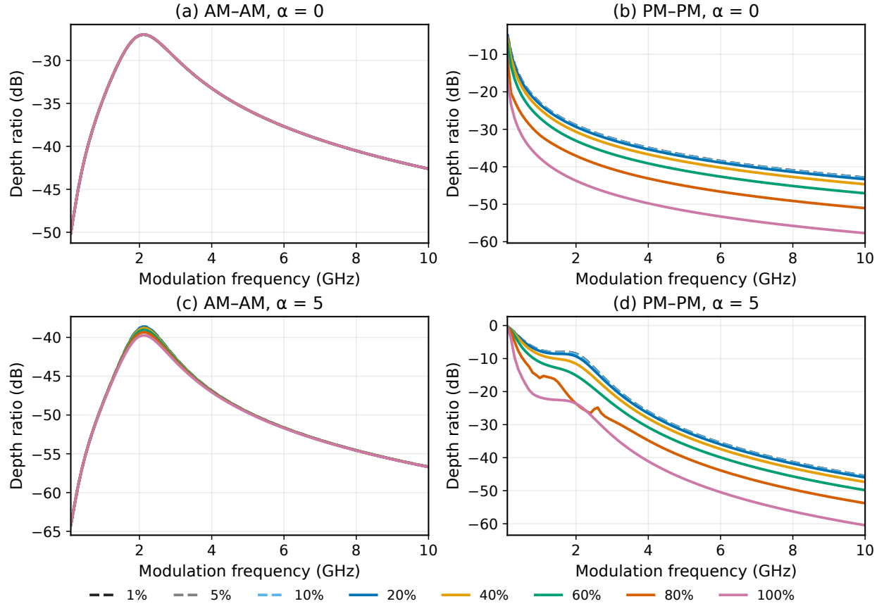
FIG. 5. Modulation responses over an extended selection of depths. AM \rightarrow AM and PM \rightarrow PM fundamental responses at R_{\text{inj}} = -50 dB and zero detuning for a,b) \alpha = 0 and c,d) \alpha = 5 . Curves correspond to depths of 1%, 5%, 10%, 20%, 40%, 60%, 80%, and 100%.
