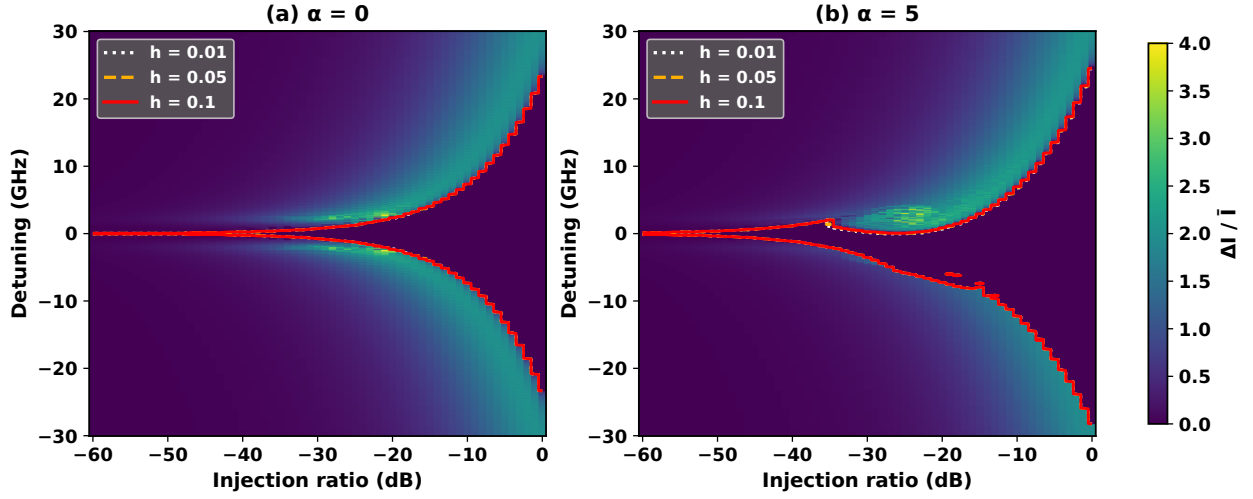
FIG. 4. Sensitivity of the joint-region contours to the metric cutoffs. Relative intensity-swing maps for a) \alpha = 0 and b) \alpha = 5 . Contours satisfy both \Delta I / \bar{I} \leq h and \Delta \phi \leq h rad for h = 0.01, 0.05 , and 0.10 .
