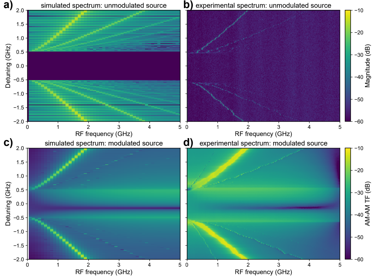
FIG. 6. Comparison of fiber measurements and simulation. Unmodulated injection: a) simulated injected-laser intensity spectrum and b) spectrum measured in SVA spectrum mode. Modulated injection: c) simulated amplitude response and d) response measured in VNA mode after reference subtraction and optical-power normalization. The simulated fractional field-amplitude response at the drive frequency is divided by the input AM depth. Horizontal and vertical axes show RF frequency and optical detuning, respectively. All panels use color limits of -60 to -10 dB, with spectral normalization in the upper row and transfer-function normalization in the lower row.
