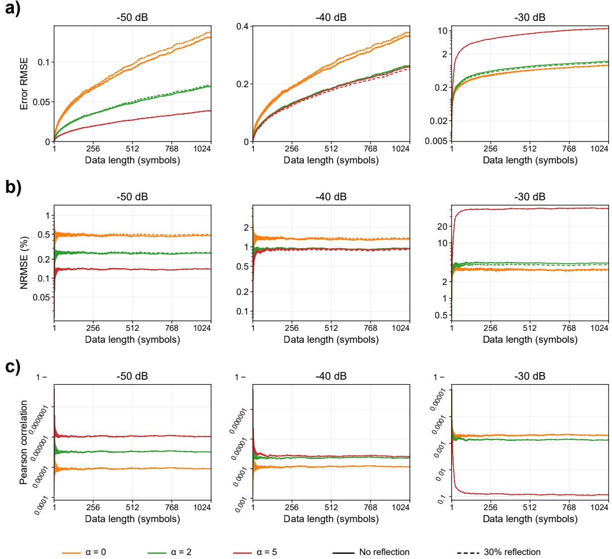
FIG. 9. Accumulation accuracy versus encoded sequence length. a) RMSE, b) NRMSE (%), and c) Pearson correlation over the first L = 1 –1024 symbols of the inputs in Fig. 8. Columns correspond to injection ratios of -50 , -40 , and -30 dB; orange, green, and red denote \alpha = 0, 2, 5 , respectively. Solid and dashed curves denote R_f = 0 and 0.30 . Each subplot uses its own vertical range. RMSE is plotted on linear axes at -50 and -40 dB and a logarithmic axis at -30 dB; NRMSE uses logarithmic axes. In (c), tick labels express correlation as 1 - r_p beneath a 1 - prefix, with logarithmic spacing in 1 - r_p .
