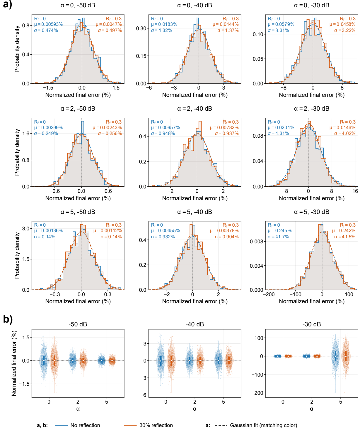
FIG. 8. Final accumulated-error distributions for 1000 input pairs at L = 1024 . Errors are normalized according to Eq. (9). a) Histograms with Gaussian fits (dashed curves); fitted means \mu and standard deviations \sigma are given in percentage points. Rows correspond to \alpha = 0, 2, 5 . b) Error distributions versus \alpha , with individual inputs shown as dots, density as violins, interquartile ranges as thick bars, and medians as white dots. Columns correspond to injection ratios of -50 , -40 , and -30 dB. Blue and orange denote R_f = 0 and 0.30 , respectively.
