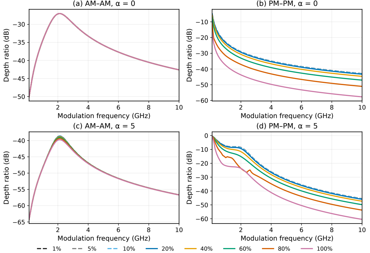
FIG. 5. Expanded depth selection from the Fig. 5 sweeps. AM→AM and PM→PM fundamental responses at R_{\text{inj}} = -50 dB and zero detuning for a,b) \alpha = 0 and c,d) \alpha = 5 . The displayed depths are 1%, 5%, 10%, 20%, 40%, 60%, 80%, and 100%; the underlying grid contains every 1% increment.
