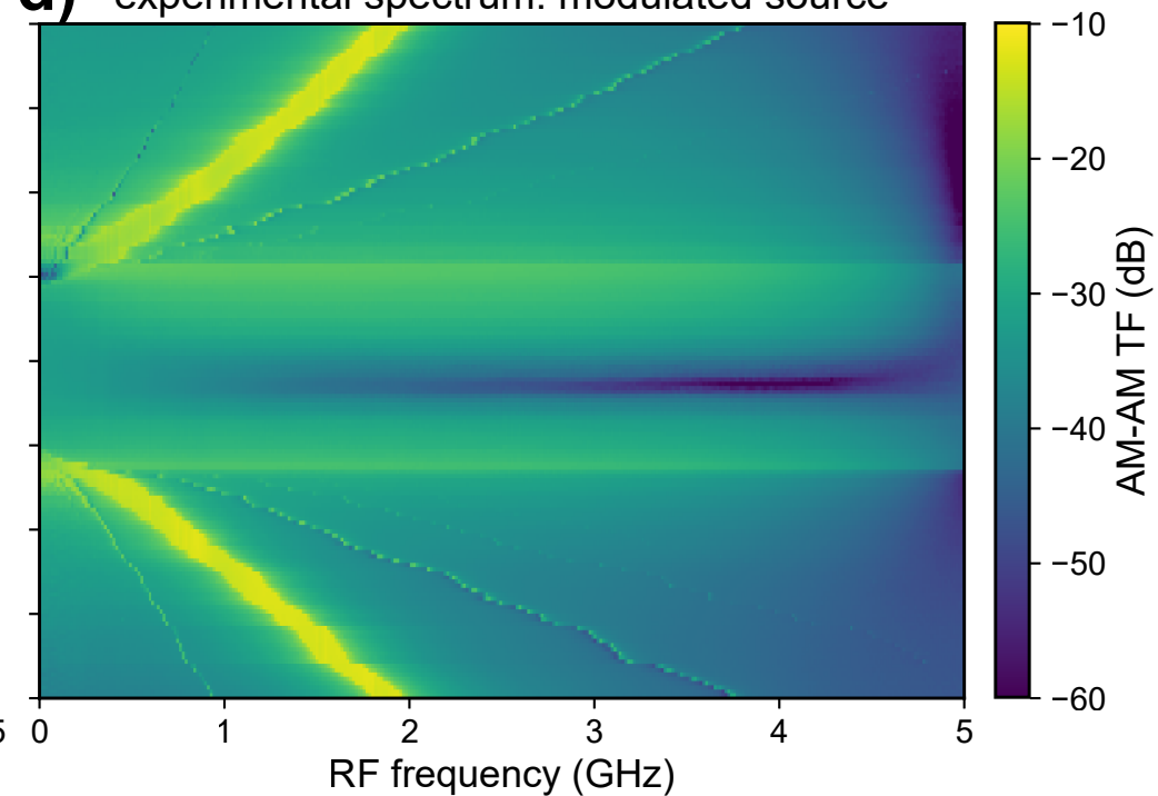
d) experimental spectrum: modulated source
