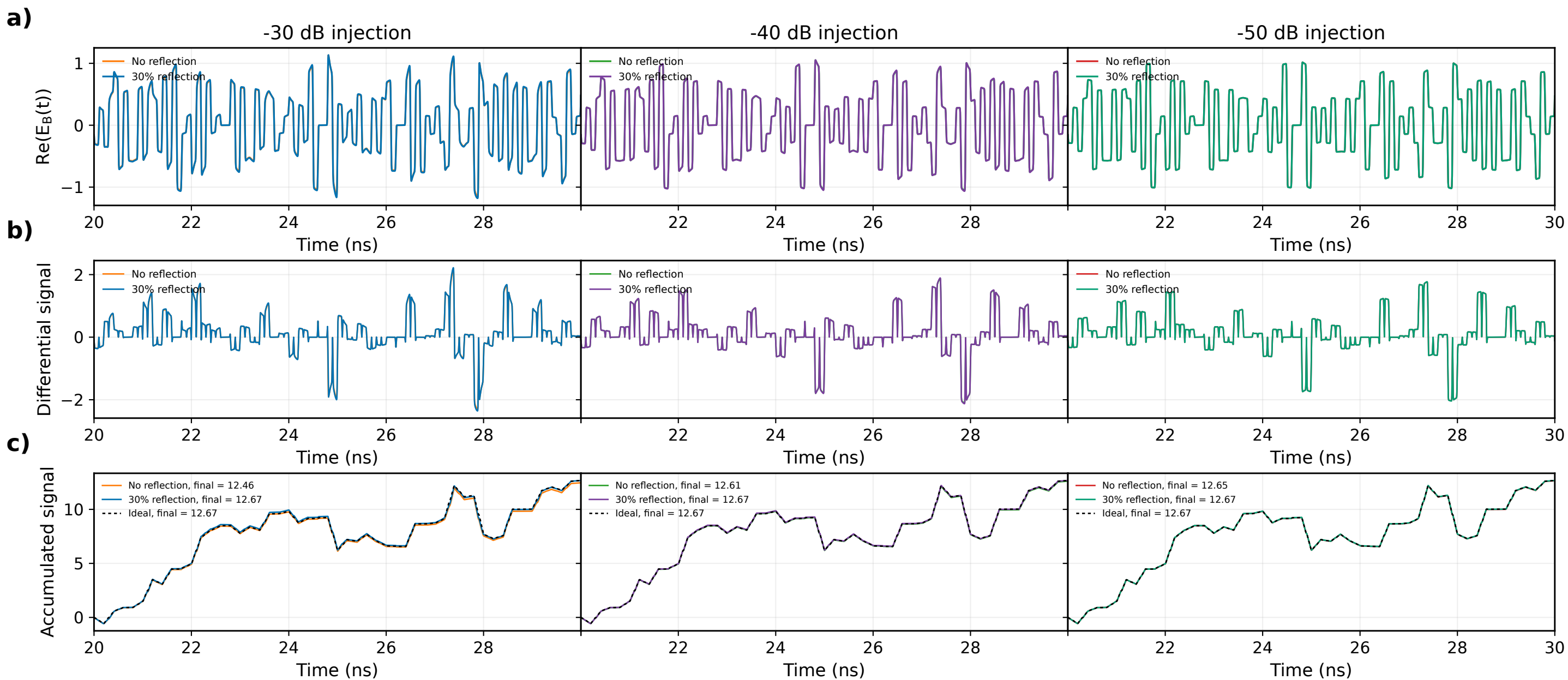
Supplementary Fig. 7: matched main-text sequence with 30% output reflection
