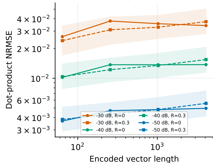
(a) \alpha = 0
