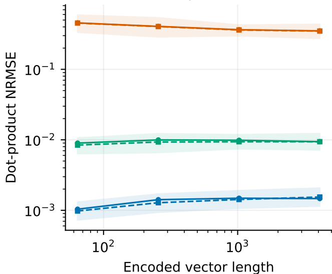
(b) \alpha = 5
