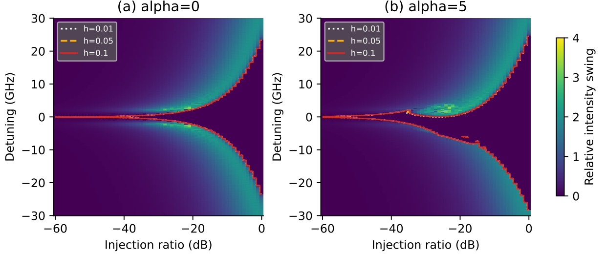
FIG. 4. Empirical cutoff comparison. Intensity-swing maps for a) \alpha = 0 and b) \alpha = 5 , with contours of the joint conditions \Delta I / \bar{I} \leq h and \Delta \phi \leq h rad at h = 0.01, 0.05 , and 0.10 . Color represents the original relative intensity swing. The comparison assesses the descriptive contour, rather than proving dynamical stability.
