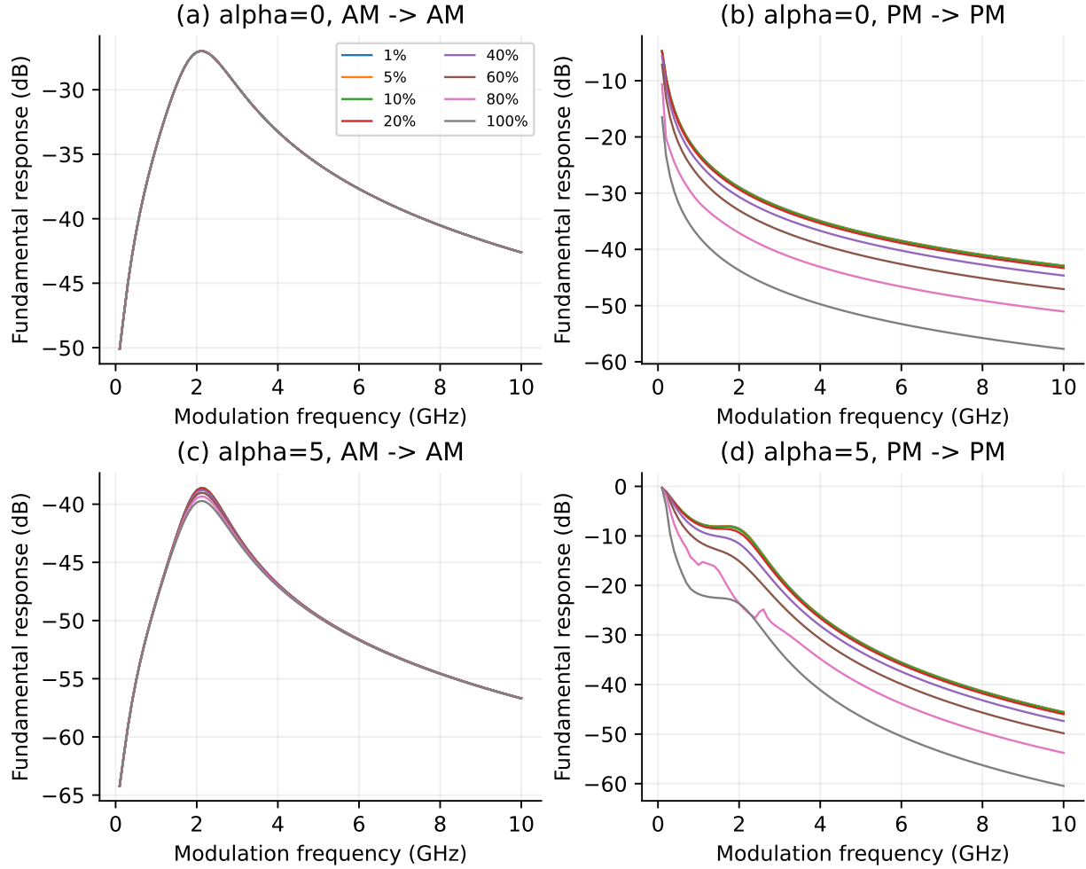
FIG. 5. Expanded depth selection from the Fig. 5 sweeps. AM \rightarrow AM and PM \rightarrow PM fundamental responses at R_{\text{inj}} = -50 dB and zero detuning for a,b) \alpha = 0 and c,d) \alpha = 5 . The displayed depths are 1%, 5%, 10%, 20%, 40%, 60%, 80%, and 100%; the underlying grid contains every 1% increment.
