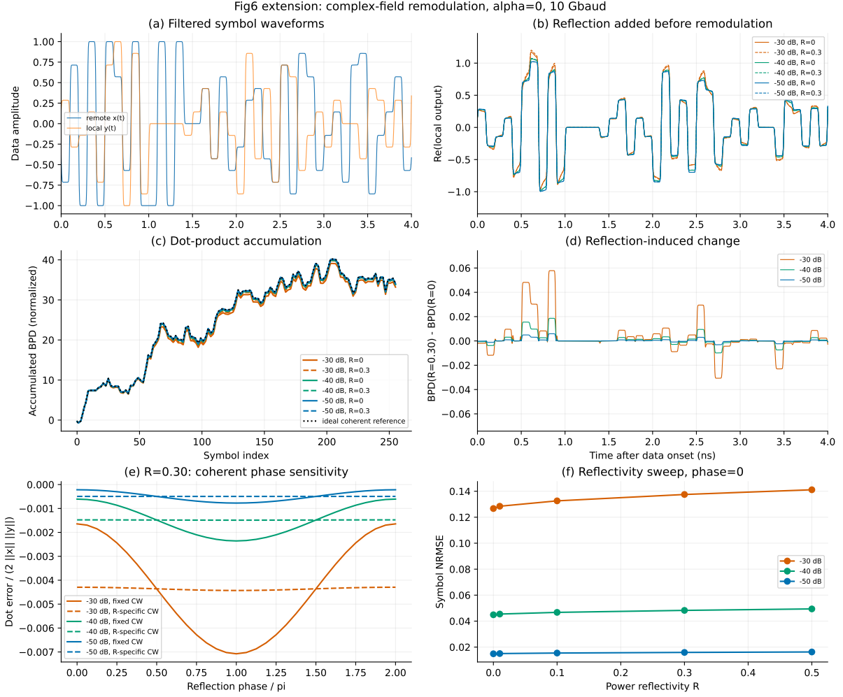
FIG. 6. Output reflection before local remodulation. Example at \alpha = 0 , 10 Gbaud, and 256 encoded symbols. a) Filtered remote and local data. b) Locally remodulated field with R_f = 0 and 0.30. c) Running dot product. d) Reflection-induced change in the differential signal. e) Reflection-phase dependence at R_f = 0.30 , with fixed and reflection-specific CW calibration. f) Symbol-error dependence on power reflectivity at \theta_r = 0 . Reflection can add to or partially cancel an existing error; one phase or sequence does not characterize its worst-case effect.
