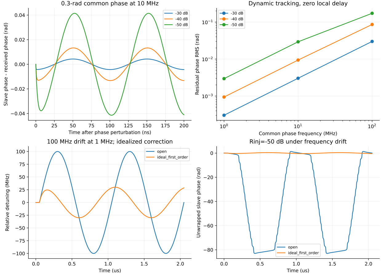
FIG. 8. Dynamic phase and detuning response. Upper left: residual phase under 0.3-rad common phase modulation at 10 MHz. Upper right: residual RMS phase versus modulation frequency for three injection ratios, with zero differential path delay. Lower left: imposed detuning before and after idealized first-order correction. Lower right: the corresponding unwrapped injected-laser phase at R_{\text{inj}} = -50 dB. The calculation illustrates phase-tracking and drift sensitivity under specified deterministic perturbations.
