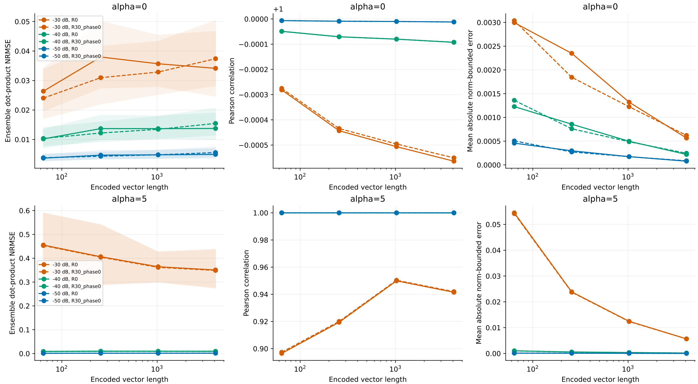
Fig6 accuracy over 32 independent sequence pairs per length (bands: bootstrap 95% CI)
