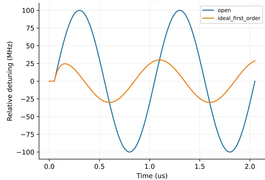
100 MHz drift at 1 MHz; idealized correction
