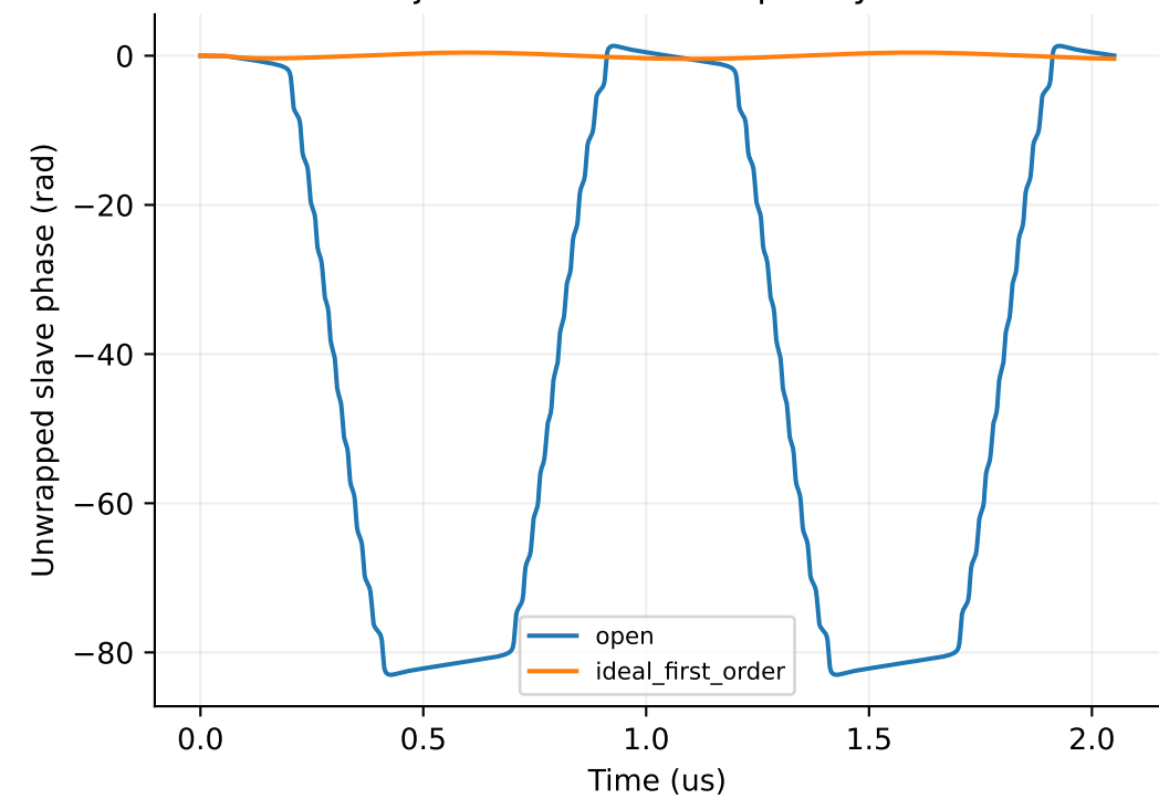
Rinj=-50 dB under frequency drift
