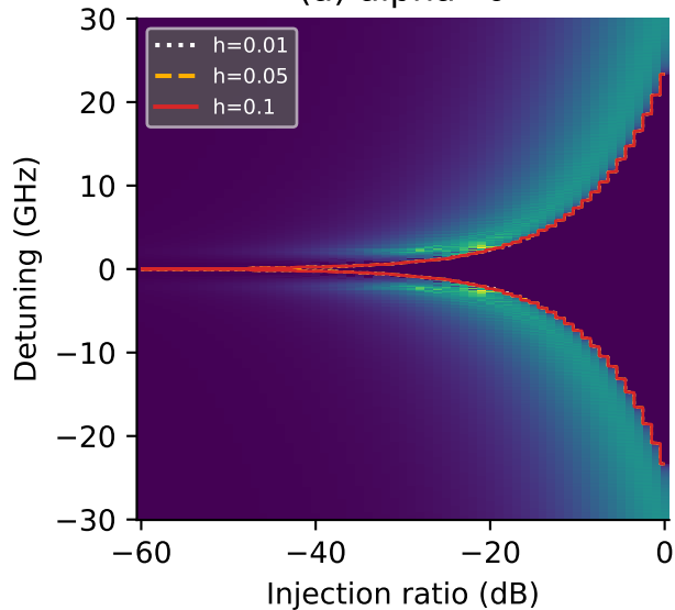
(a) \alpha=0
