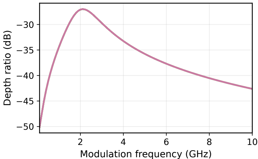
(c) AM-AM, \alpha = 5
