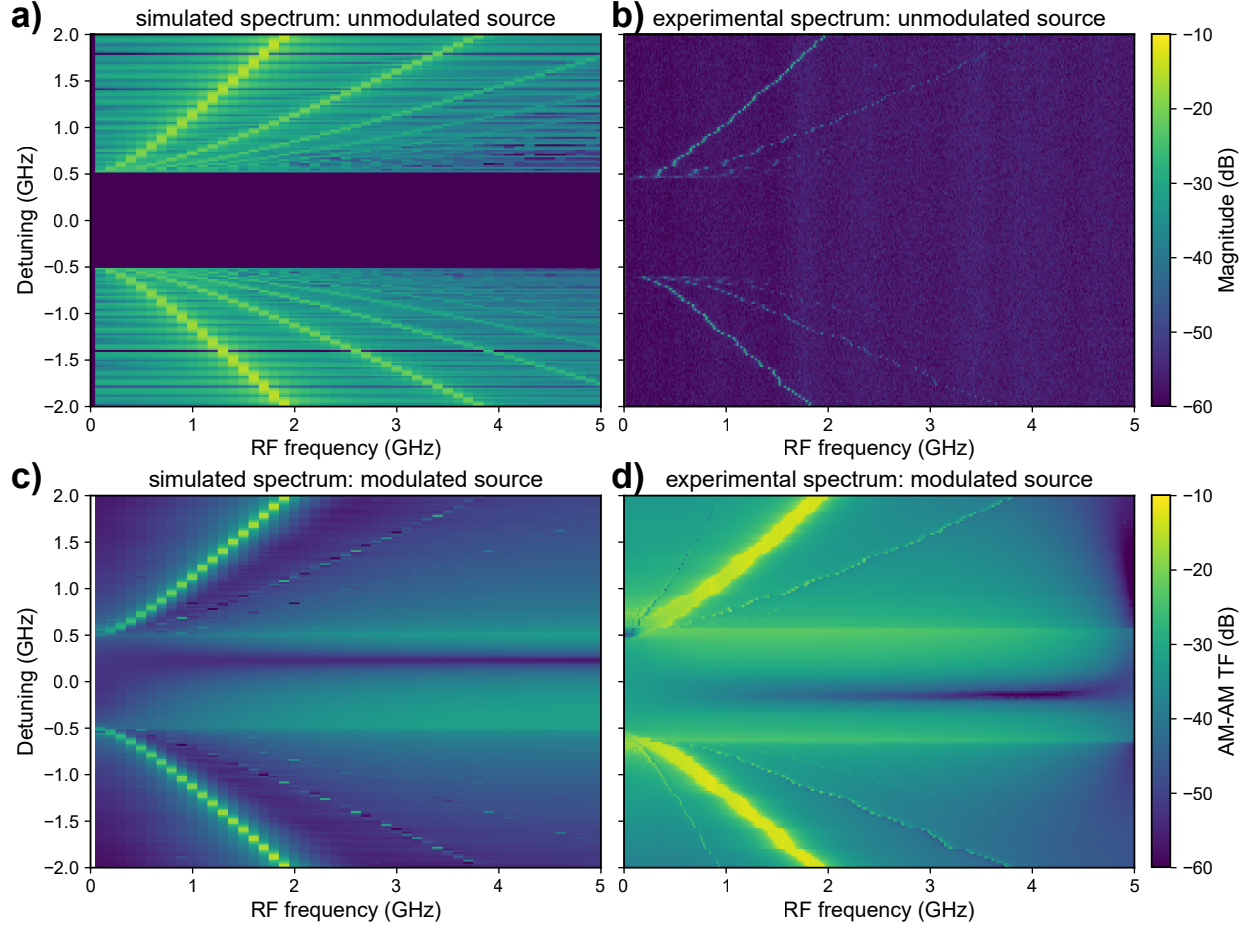
FIG. 9. Simulation and experiment comparison heatmaps. The first row shows unmodulated injection: a) simulated RF FFT spectrum of the injected-laser output intensity and b) experimental injected-laser RF spectrum measured in SVA spectrum mode. The second row shows modulated injection: c) simulated AM-to-AM transfer function and d) experimental AM-to-AM transfer function measured in VNA mode after reference subtraction and optical-power normalization. The horizontal axis is RF spectral frequency in (a,b) and applied RF modulation frequency in (c,d); the vertical axis is optical detuning. All maps use common displayed color limits of -60 to -10 dB, with spectral magnitude and transfer-function normalization as indicated by the color bars. Simulations use \alpha = 2 , threshold = 1.944, and R_{\text{inj}} = -40 dB; measurements use the external -15 dB condition.
