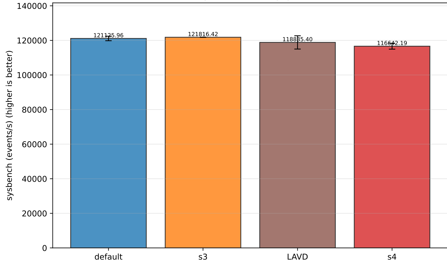
Sysbench Throughput
