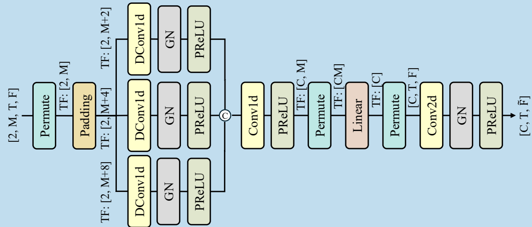
(c) Circular Array Spatial Processor (CASP)
