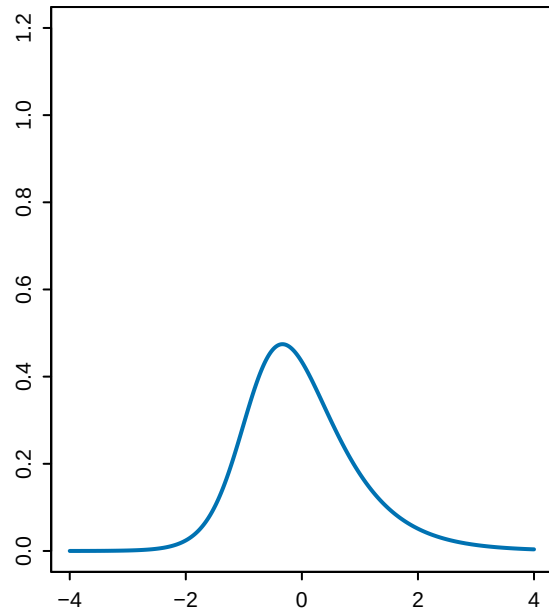
2) Fleishman polynomial a=-0.127, b=0.872, c=0.127, d=0.036 ; skew 0.50, ex.kurt 1.00
