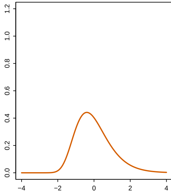
4) Fleishman polynomial a=-0.136, b=0.942, c=0.136, d=0.013 ; skew 2.00, ex.kurt 2.99
