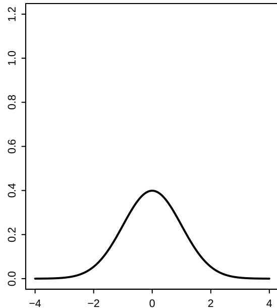
1) Normal distribution N(0, 1) ; skew 0.0, ex.kurt 0.0
