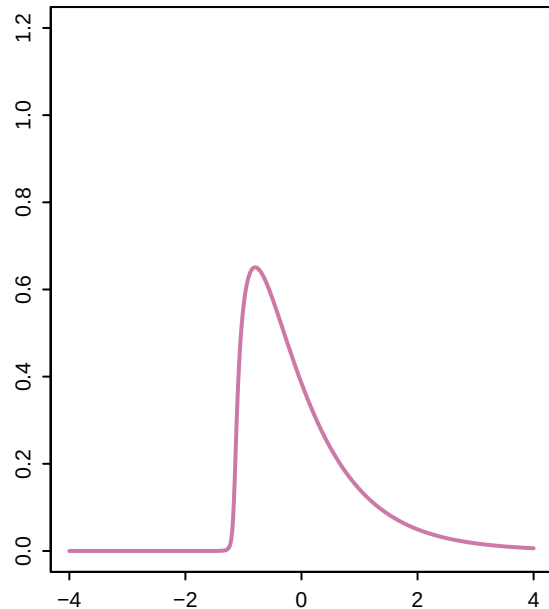
5) Fleishman polynomial a=-0.272, b=0.816, c=0.272, d=0.034 ; skew 2.00, ex.kurt 6.01
