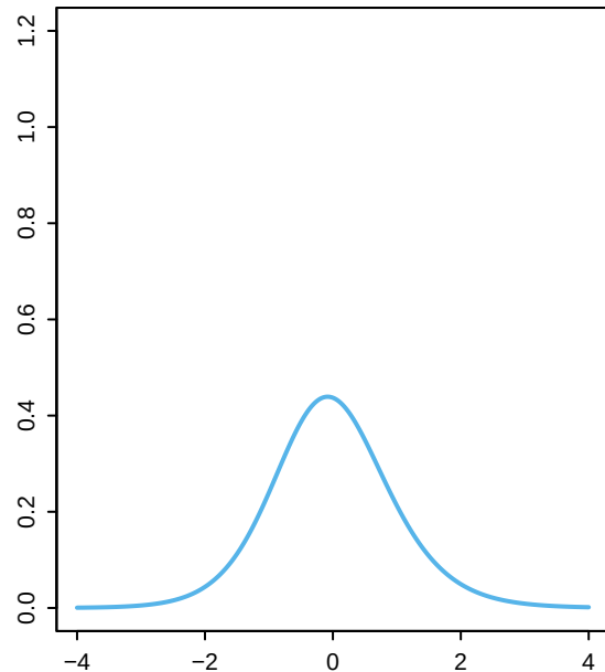
3) Fleishman polynomial a=-0.031, b=0.910, c=0.031, d=0.029 ; skew 0.50, ex.kurt 3.04
