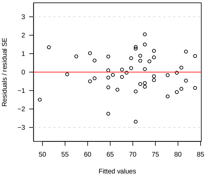
Residuals / residual SE vs. Fitted
