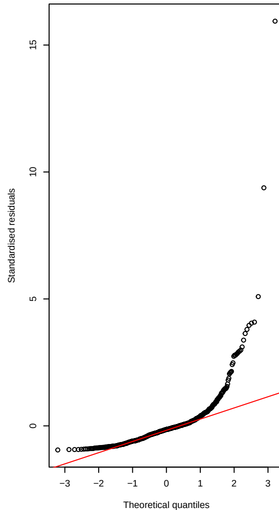
Normal Q-Q Plot
