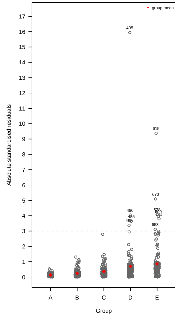
Absolute residuals vs. Group
