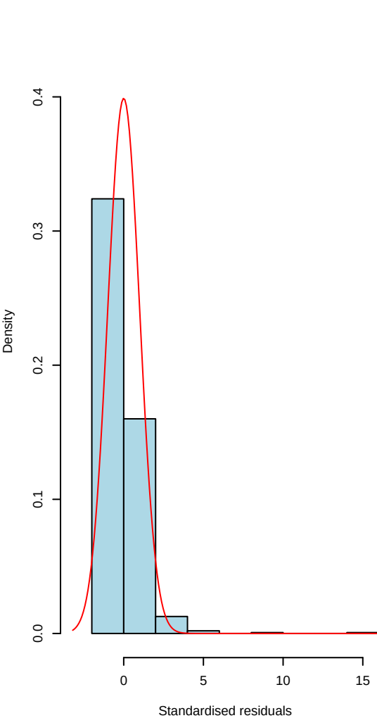
Histogram and Normal Density
