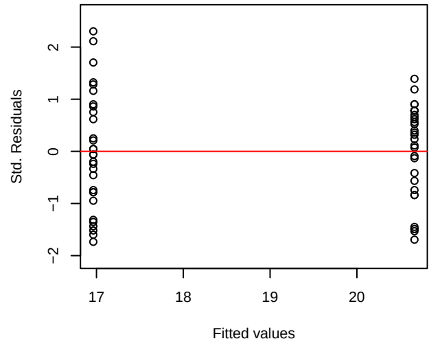
Std. Res. vs. Fitted
