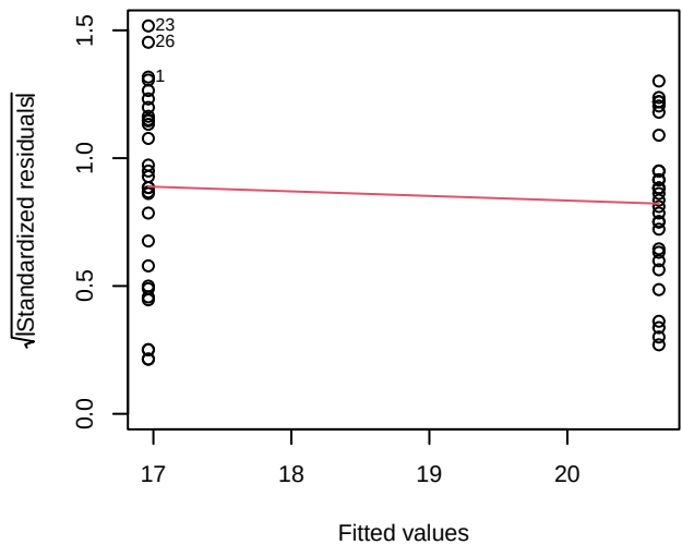
Scale-Location
