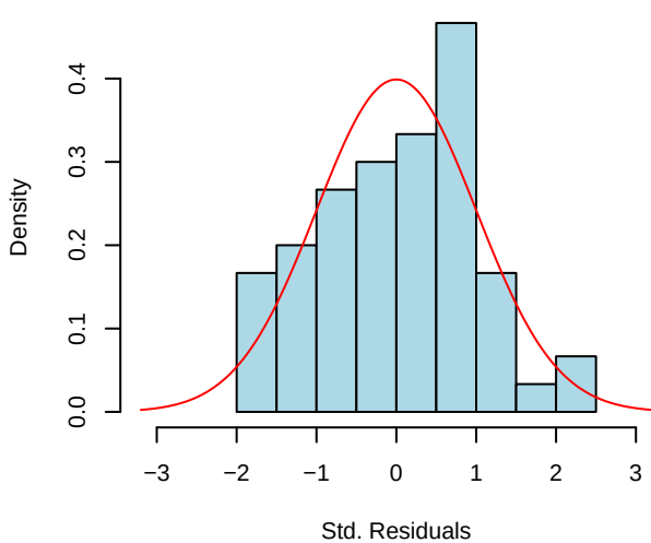
Histogram and Normal Density
