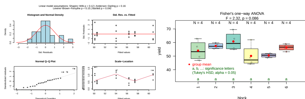
Figure 5: Fisher's one-way ANOVA applied to the npk dataset (block vs. yield). Assumption diagnostics and box plots of pea yield by experimental block; compact letter display (TukeyHSD, \alpha = 0.05 ) shows no significant pairwise differences.
