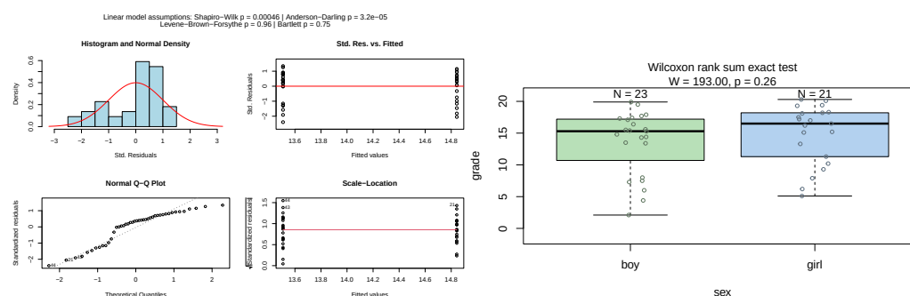
Figure 4: Wilcoxon rank-sum test applied to examination grades by sex. Assumption diagnostics (Shapiro–Wilk rejected; non-parametric path selected) and box plots with the Wilcoxon test result.
