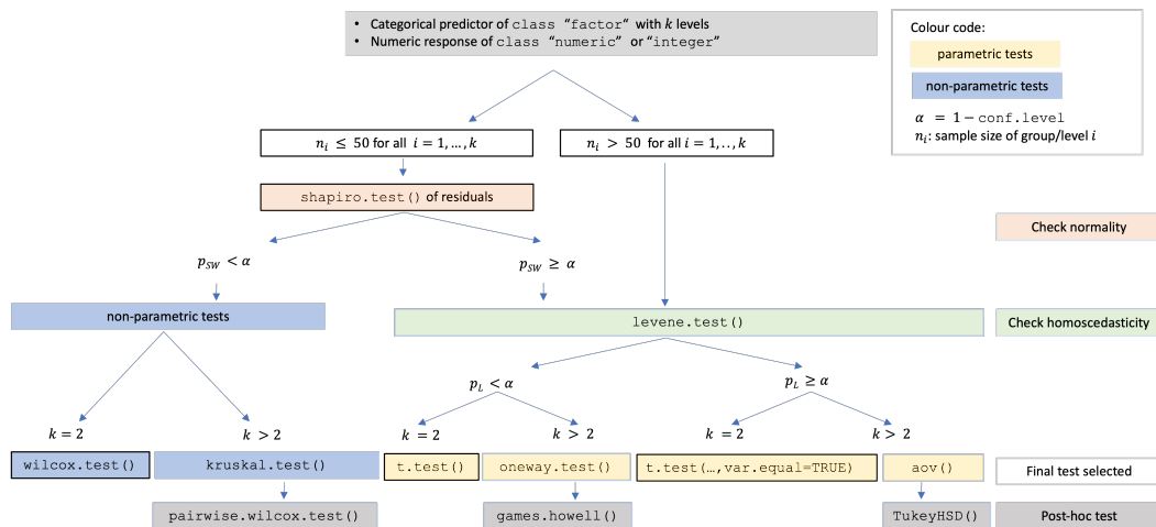
Figure 2: Decision tree for tests on central tendencies.
