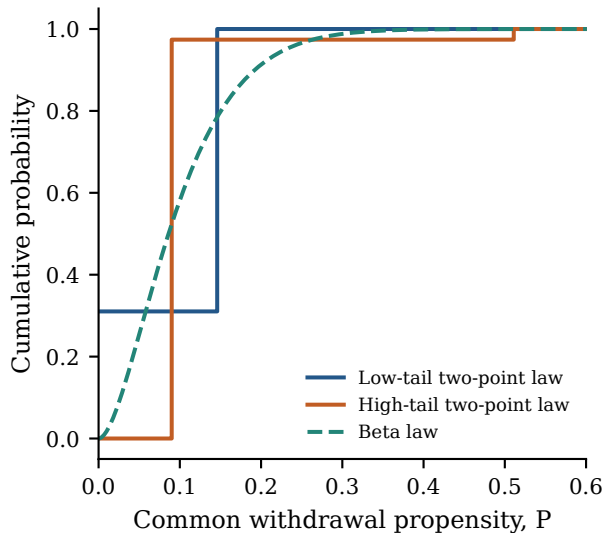
A. Identical first two moments
