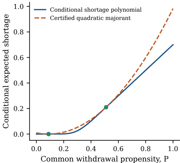
A. A global upper certificate
