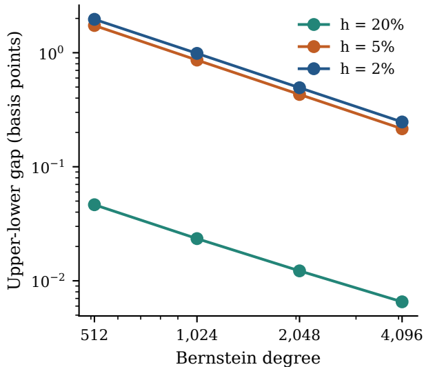
B. Numerical convergence
