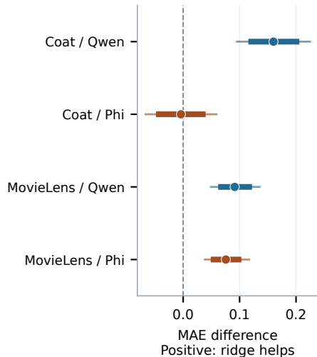
Reader choice Full minus ridge
