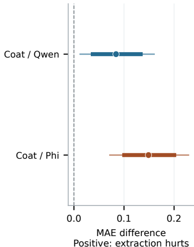
Extraction Native minus full
