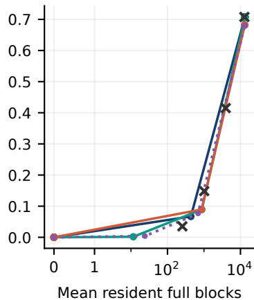
Synthetic
