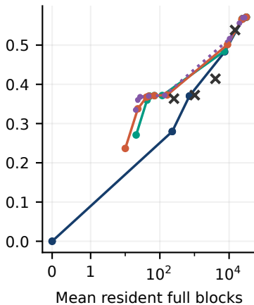
Tool agent
