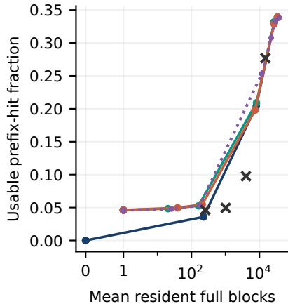
Conversation
