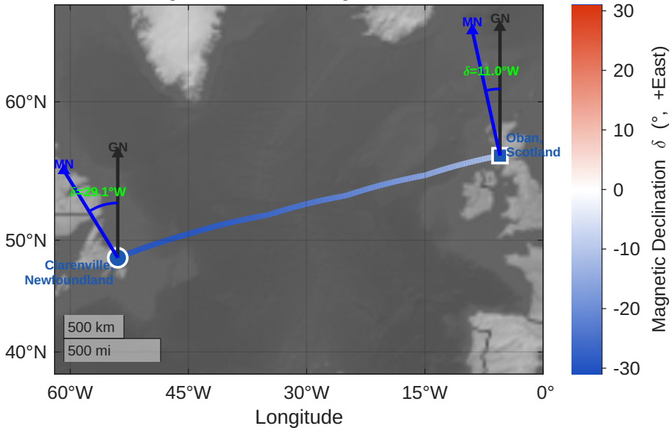
IGRF Magnetic Declination along TAT-1 Cable Route
