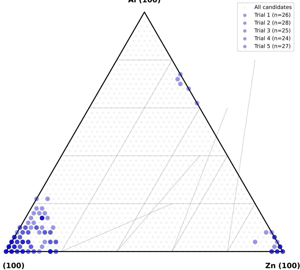
NTS conservative (batch=5) (avg 26.0 near-optimal samples)
