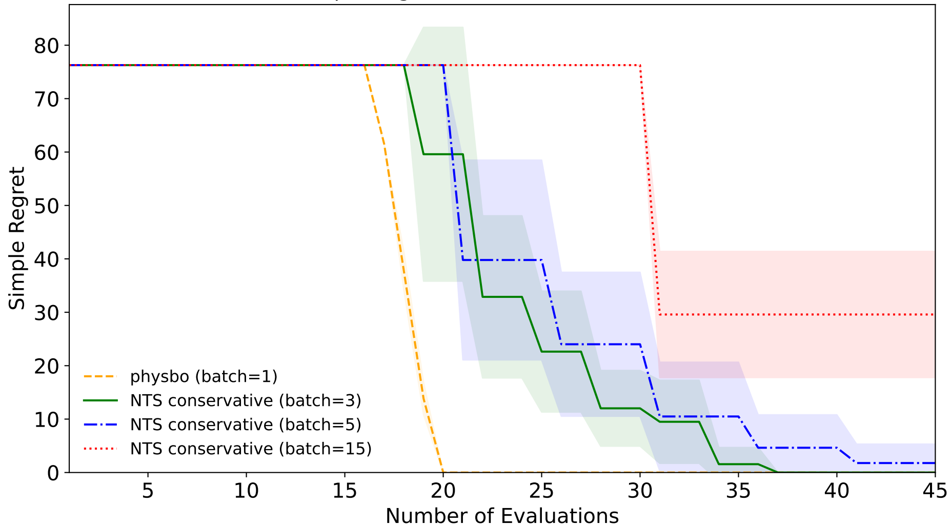
Simple Regret vs Number of Evaluations
