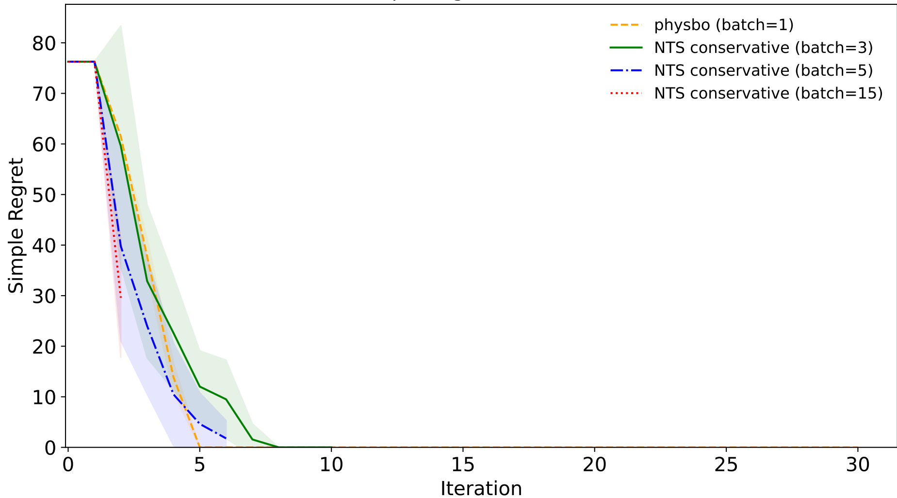
Simple Regret vs Iteration
