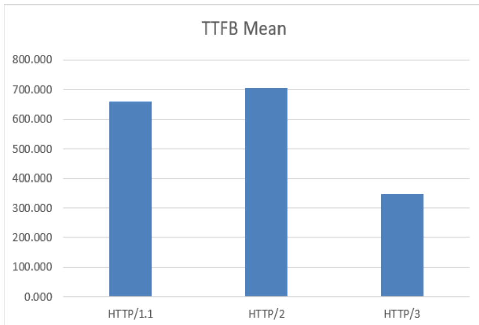
Figure 2. Average Time To First Byte (TTFB) Comparison
