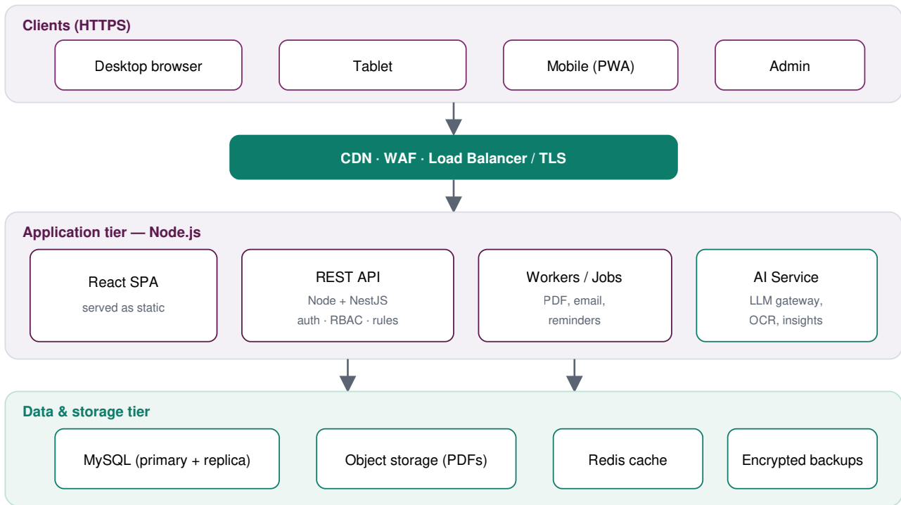
Figure 3.1 — Logical deployment architecture.
