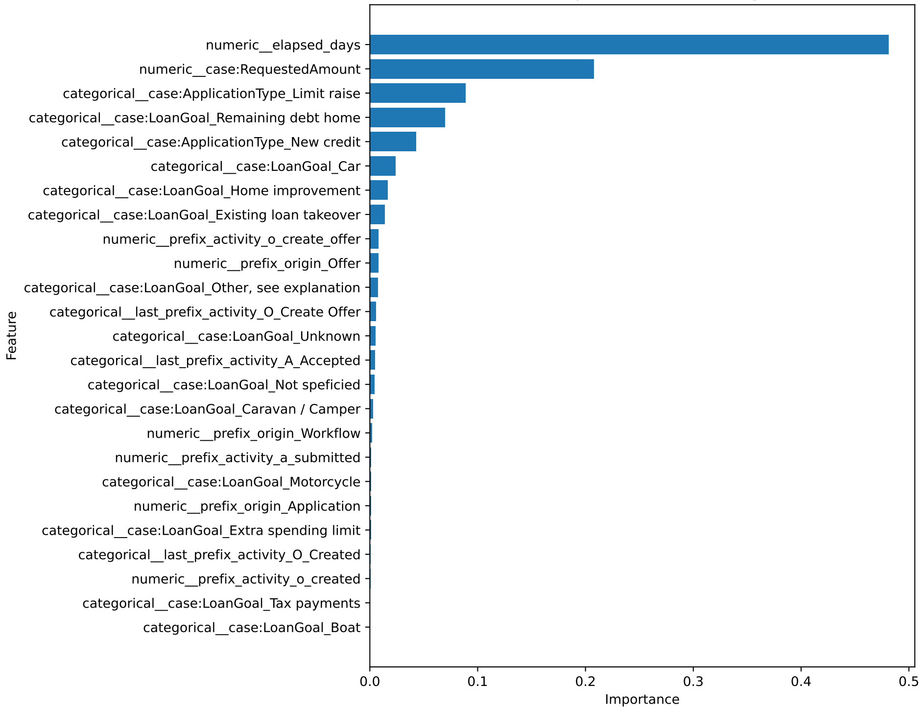
Random Forest Feature Importance for Remaining Duration Prediction
