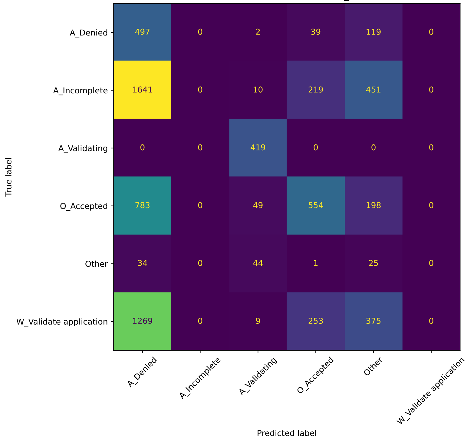
Decision Tree Confusion Matrix: O_Returned
