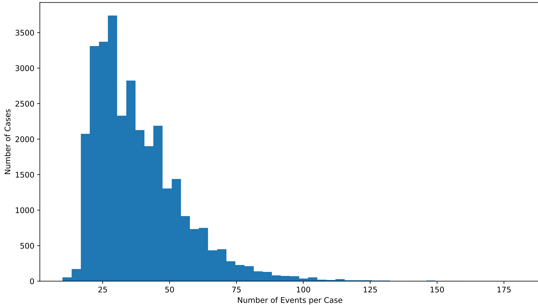
Case Length Distribution in BPIC-17 Event Log
