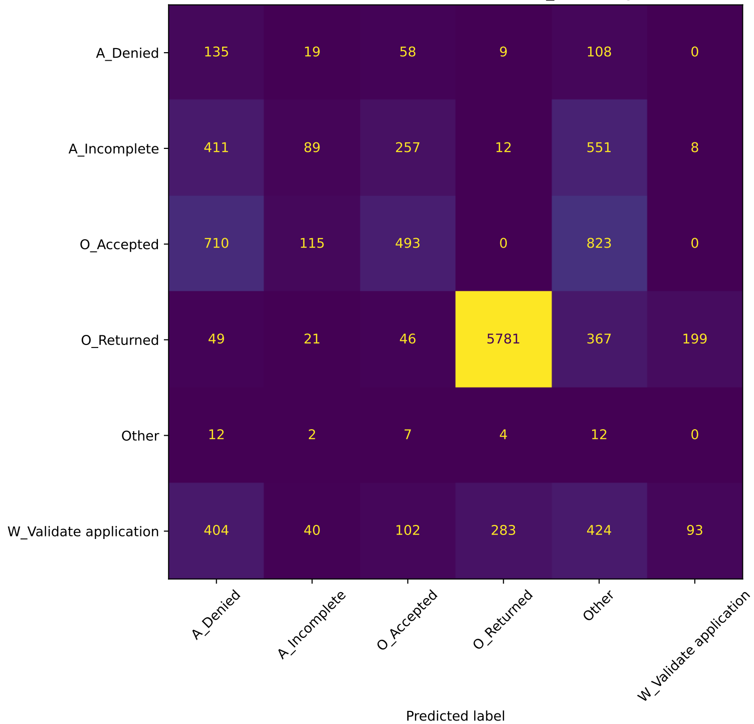
Decision Tree Confusion Matrix: A_Validating
