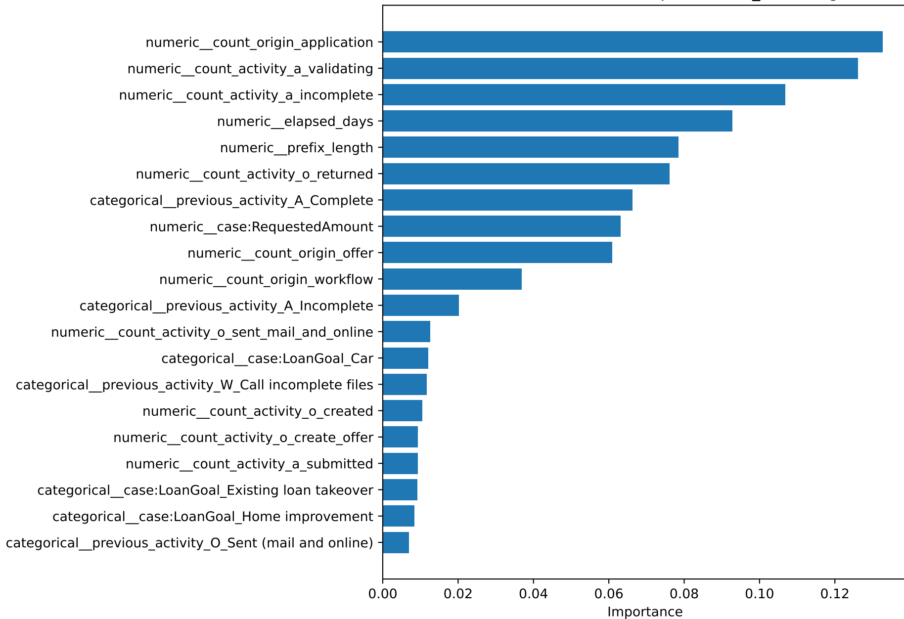
Random Forest Feature Importance: A_Validating
