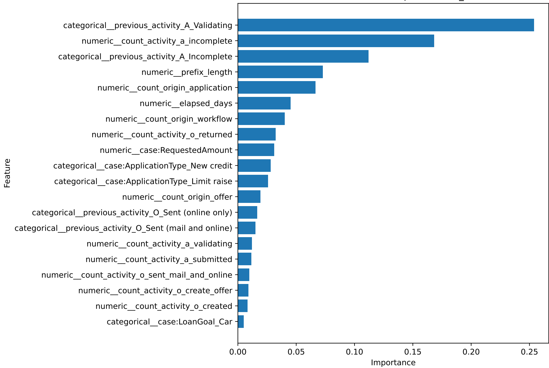
Random Forest Feature Importance: O_Returned
