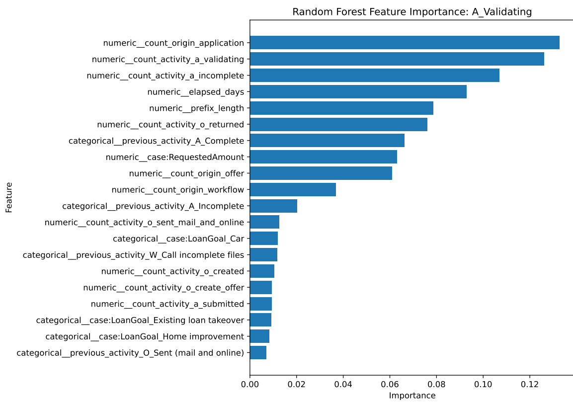
Figure 7 Feature importance for the A_Validating decision point.
