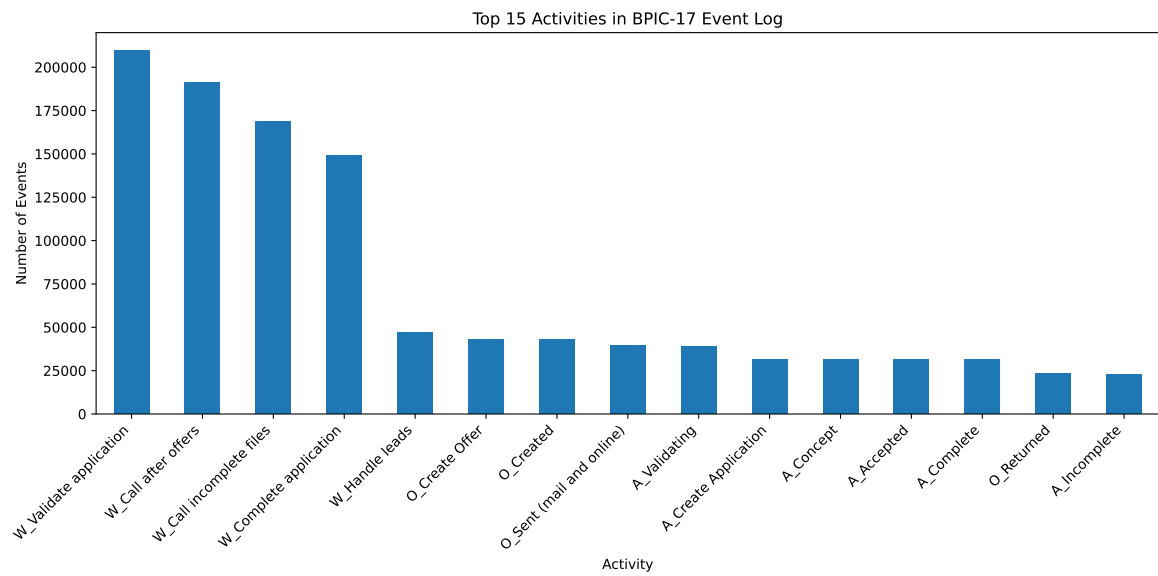
Figure 3 Top 15 activity frequencies.
