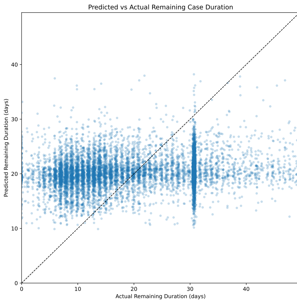
Figure 8 Predicted versus actual remaining duration.
