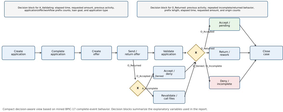
Figure 2 Compact decision-aware BPMN-style view with mined decision blocks for the two selected XOR decisions.
