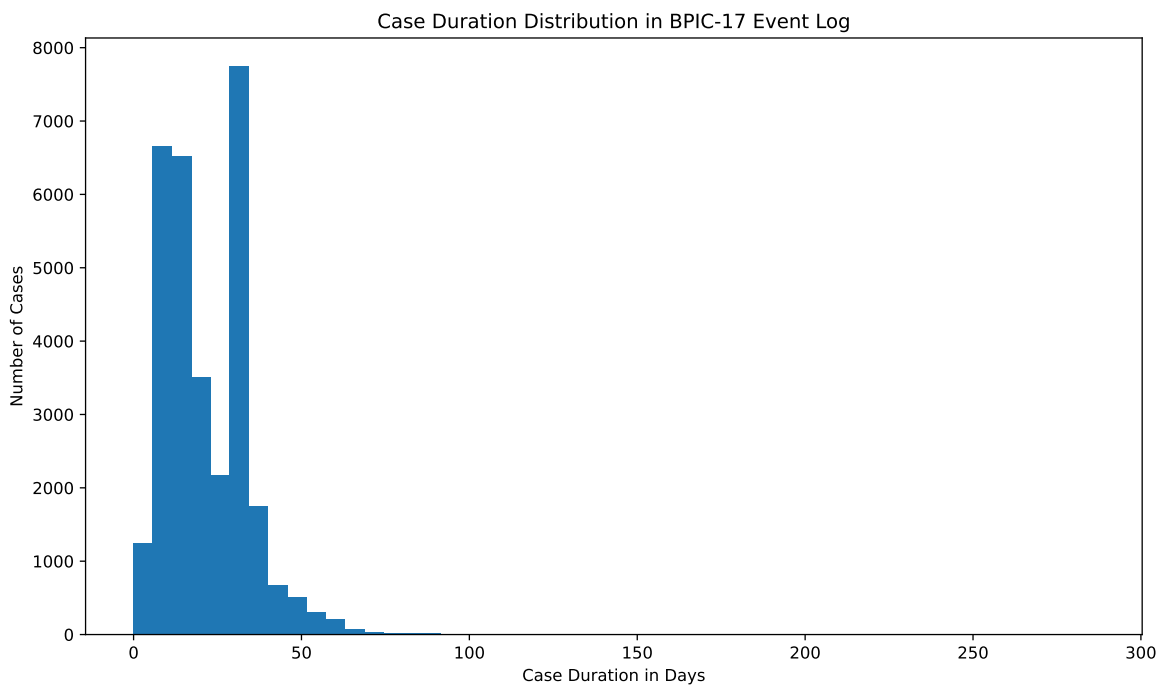
Figure 4 Case duration distribution in days.
