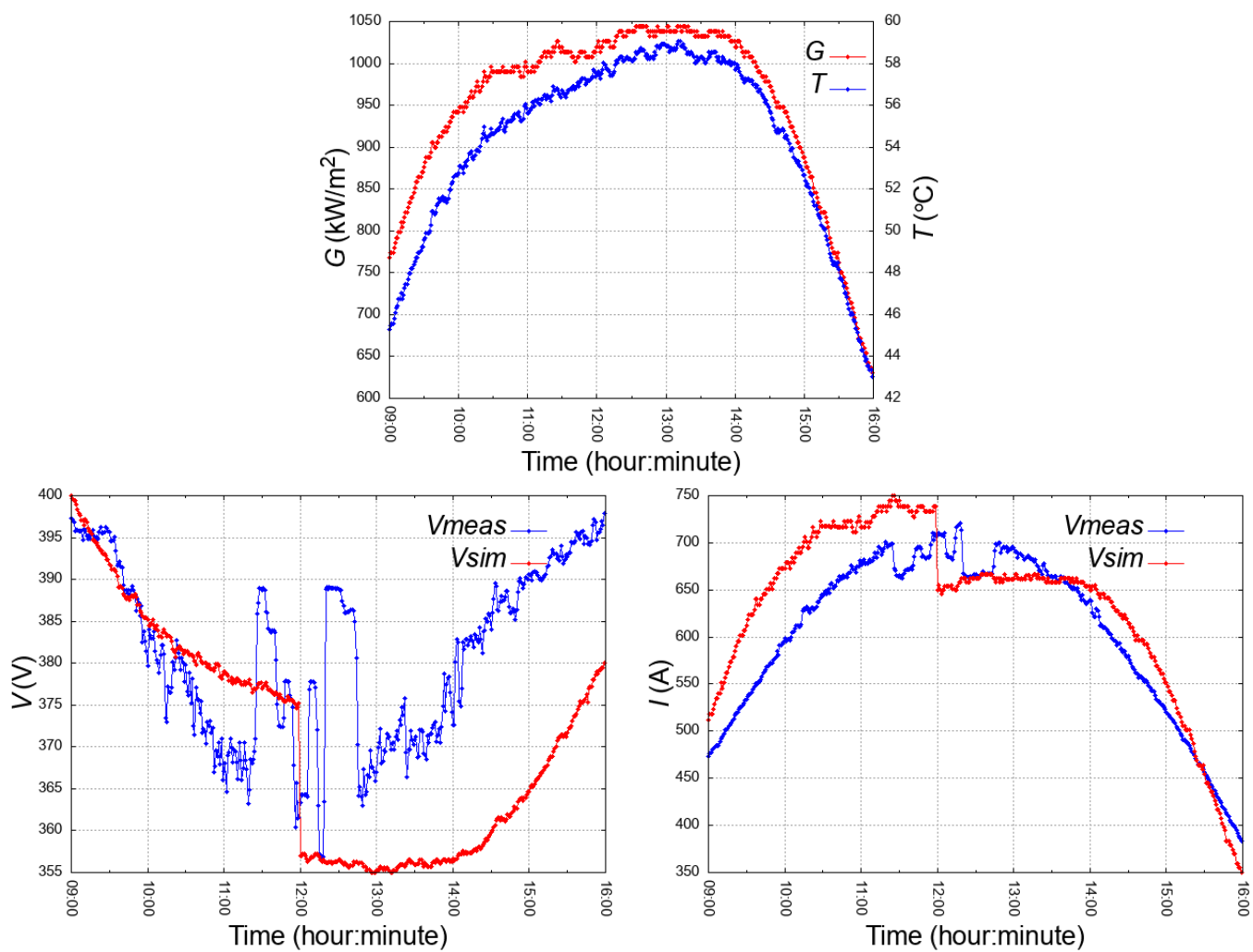
图 1 2019.5.7, 12:00 R_s=0.1 in 10 cells, 21 substrings, 20 strings
