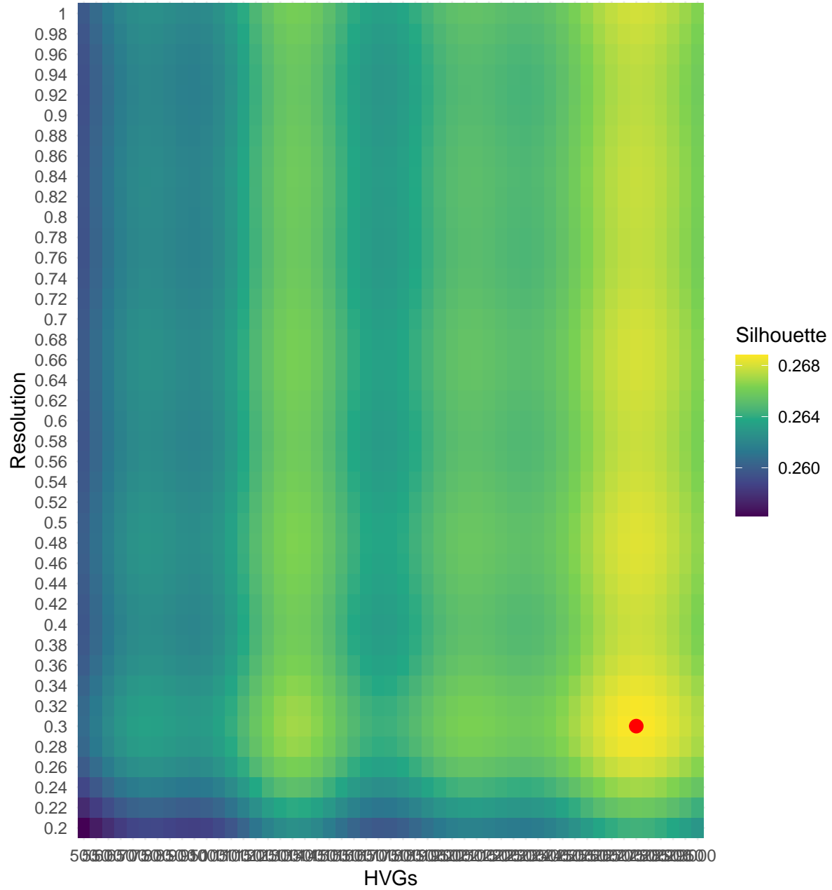
GAM-smoothed Silhouette Heatmap
